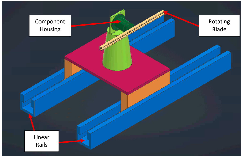
Figure 1 CAD Model of Full System Assembly Concept
